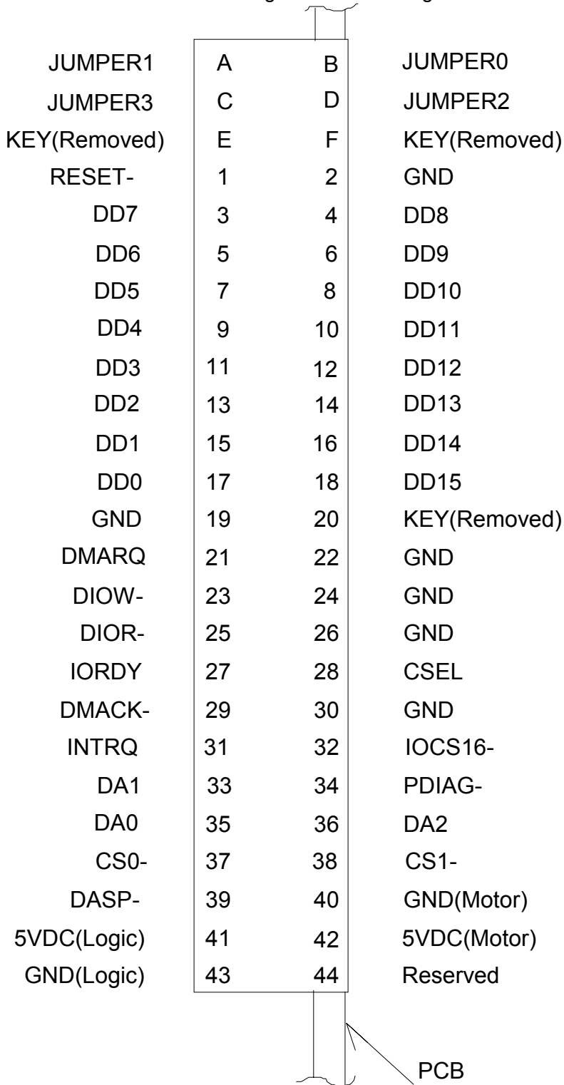
Figure 6-3 Pin Assignments
