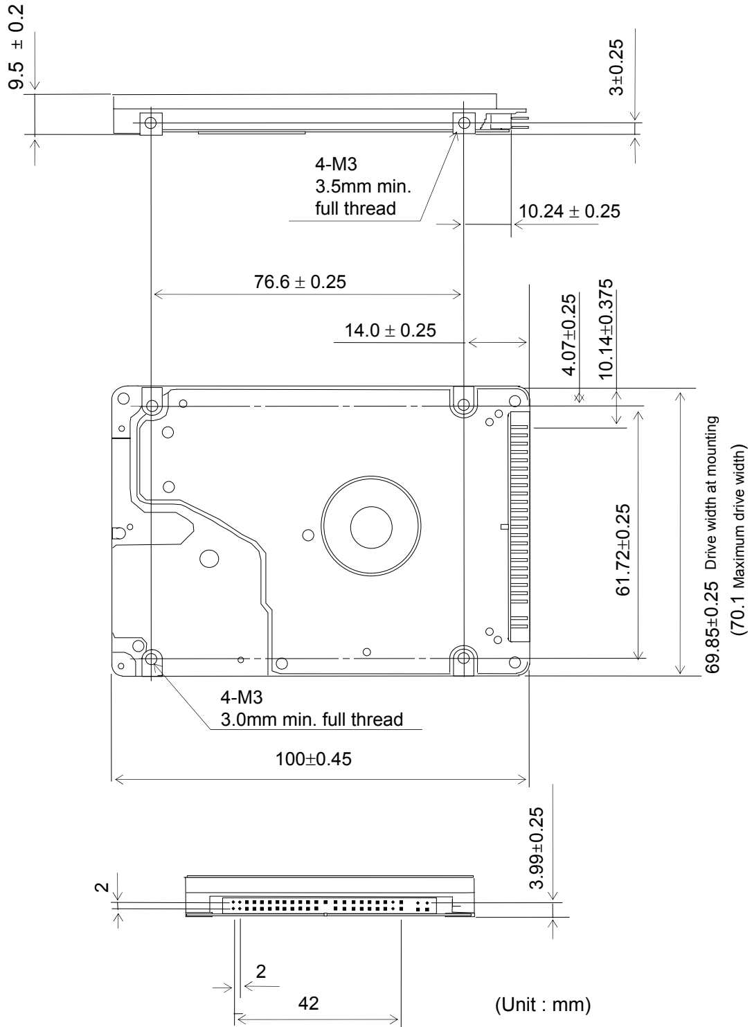
Figure 4-4 Dimensions
