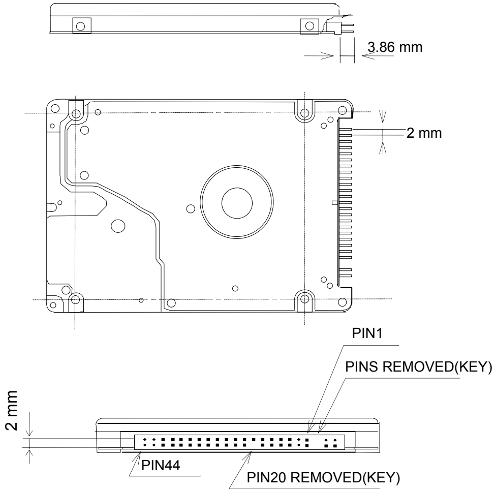
Figure 6-2 Connector Location
