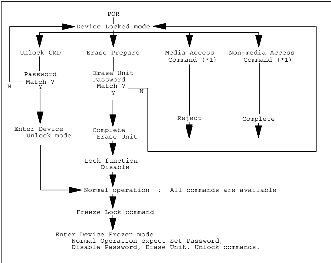
Figure 2 : Usual operation for POR
