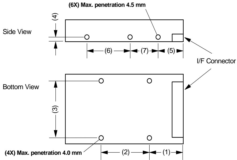
Figure 1: Mounting hole locations
