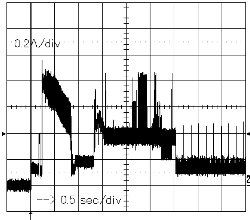
Figure 24. Typical current wave form at start up of 20 GB model)
