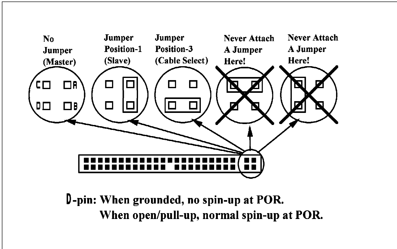
Figure 36. Address setting by a jumper for DCXA-2xxxxx.
