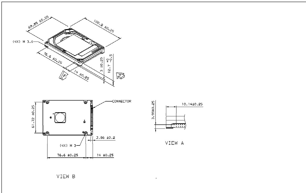
Figure 19. Outline of DCXA-2xxxxx
