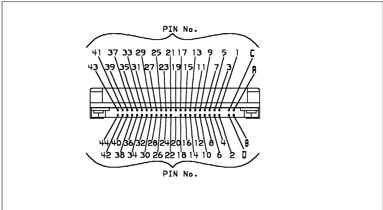
Figure 21. AT Attachment connector of DCXA-2xxxxx
